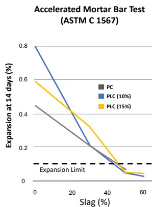
Figure 6: Expansion results from accelerated mortar bar test (left) and concrete prism test (right) from Study 4 using alkali-silica reactive siliceous limestone (Thomas et al 2010)
