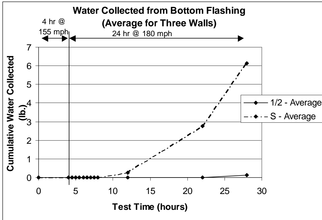
Figure 12—Test Results – Water Collected on Flashing \frac{1}{8} in. (3 mm) Skim Coat vs. \frac{1}{2} in. (13 mm) Stucco.
