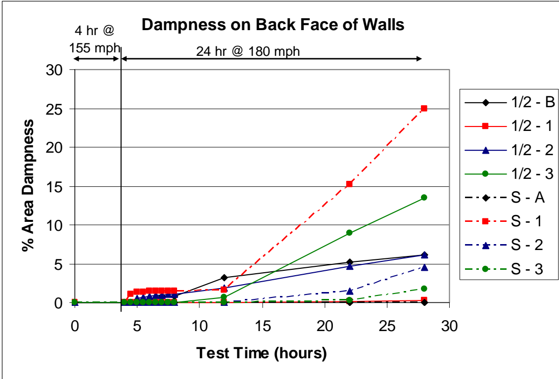
Figure 10—Area of Dampness on Leeward Wall Surface, percent
