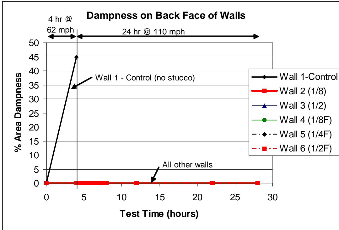
Figure 8—Area of Dampness on Leeward Wall Surface, percent
