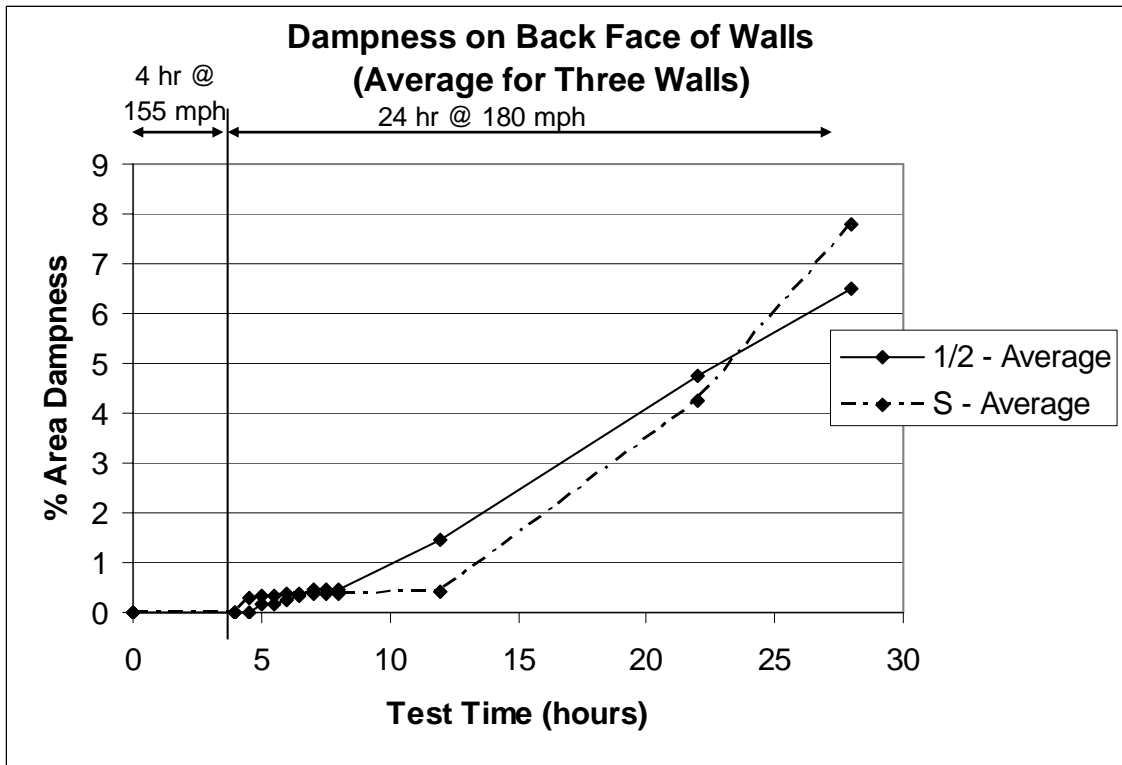
Figure 11—Test Results: Dampness 1/8 in. (3 mm) Skim Coat vs. 1/2 in. (13 mm) Stucco
