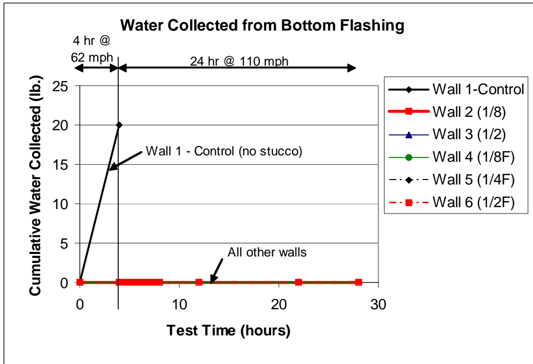
Figure 9—Test Results – Water Collected on Through-Wall Flashing, lbs.
